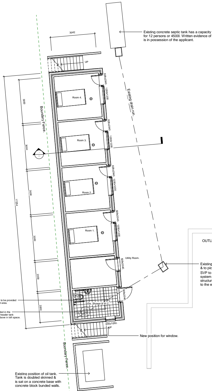
Ground floor Layout 1 : 50
