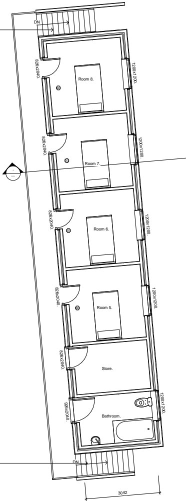
first floor Layout 1 : 50
